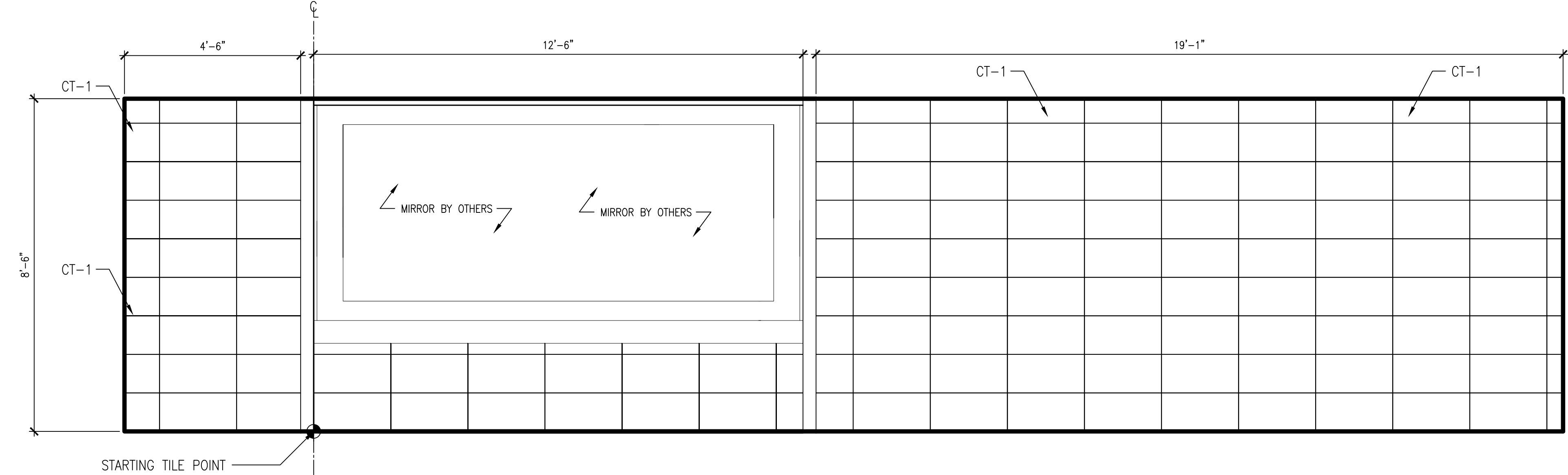
05 1/2"=1'-0" ELEVATION: SOUTH
