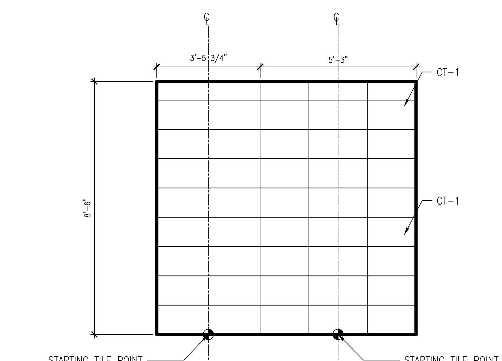
06 1/2"=1'-0" ELEVATION: WEST
