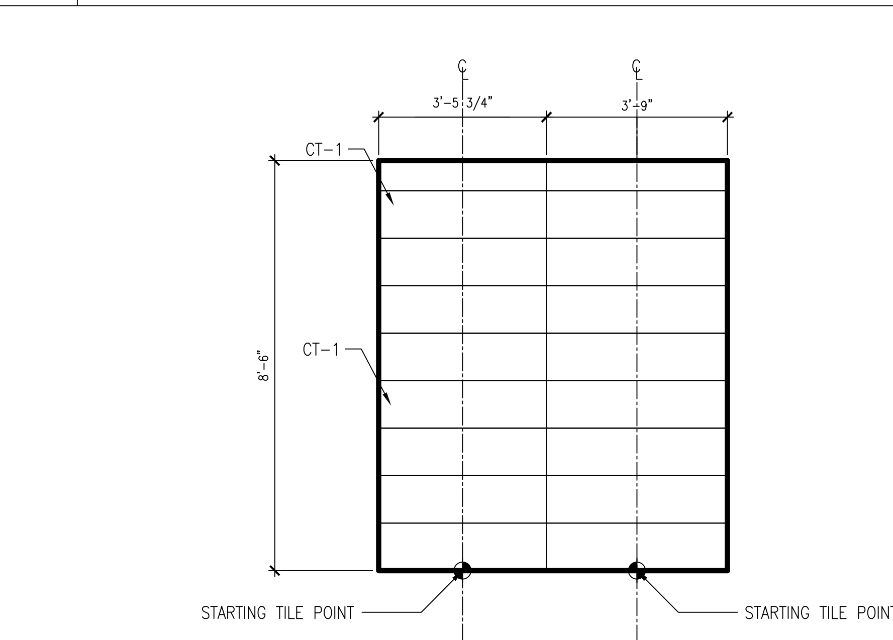
06 1/2"=1'-0" ELEVATION: WEST
