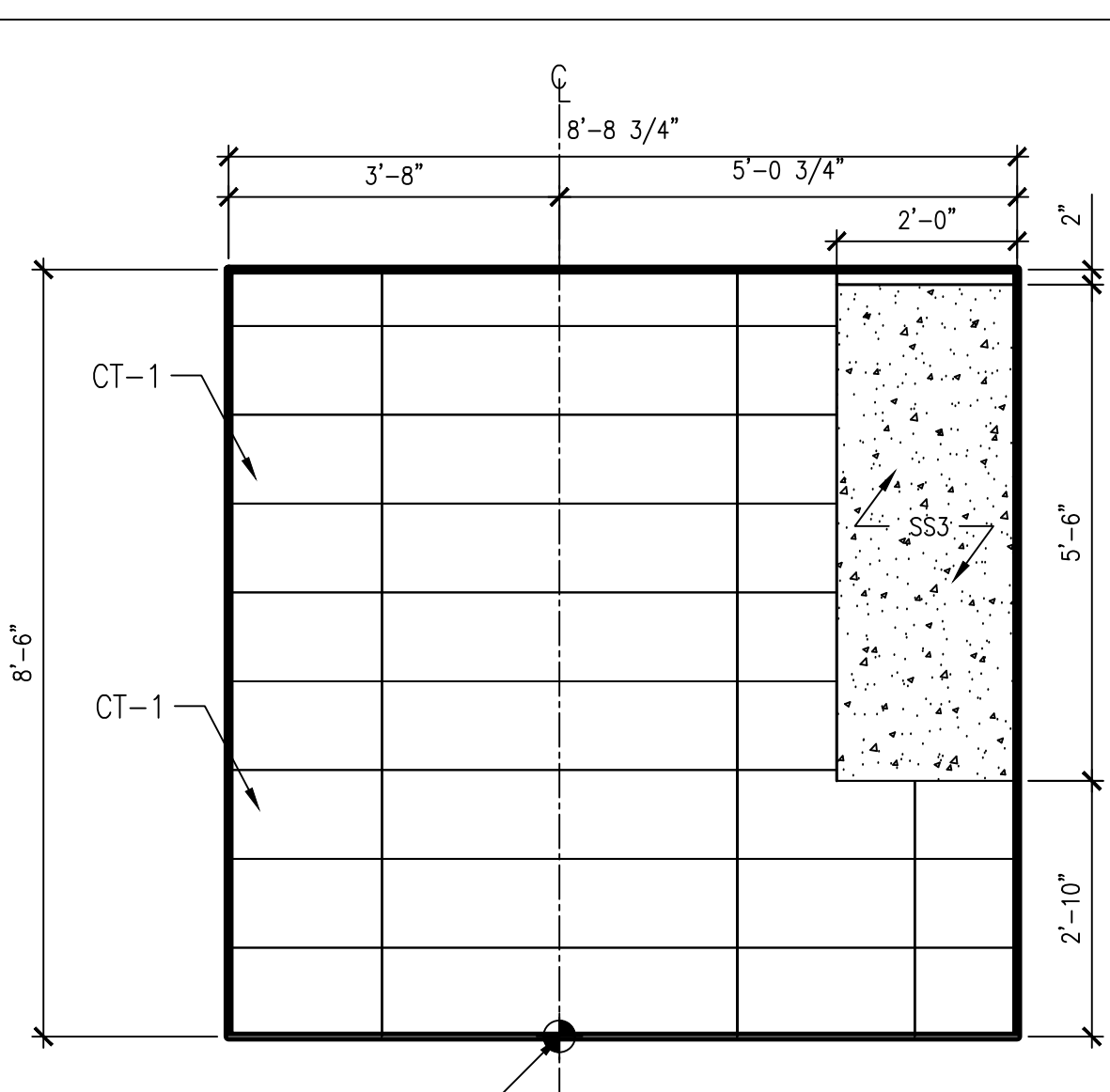
08 1/2"=1'-0" ELEVATION: EAST
