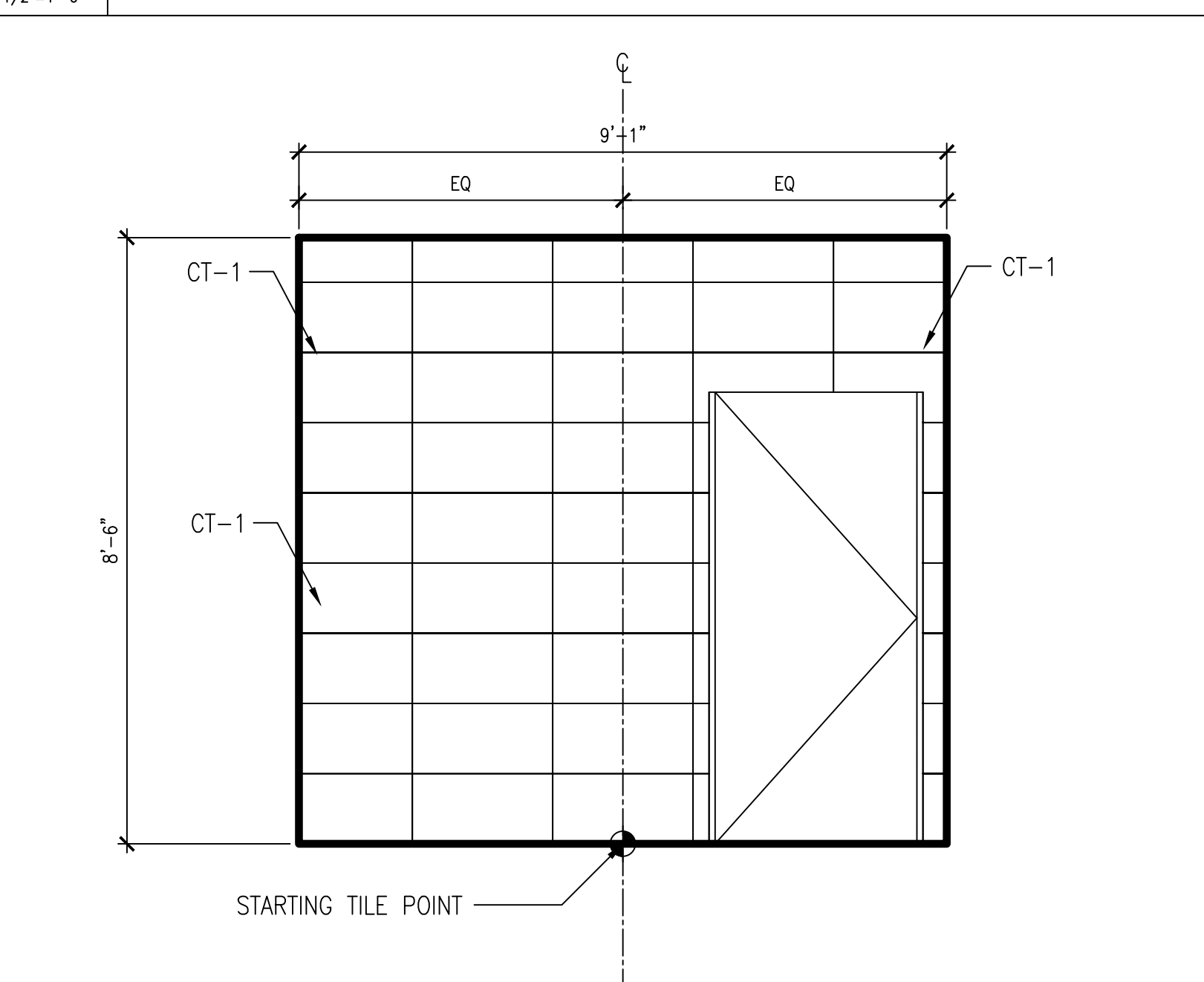
04 1/2"=1'-0" ELEVATION: EAST
