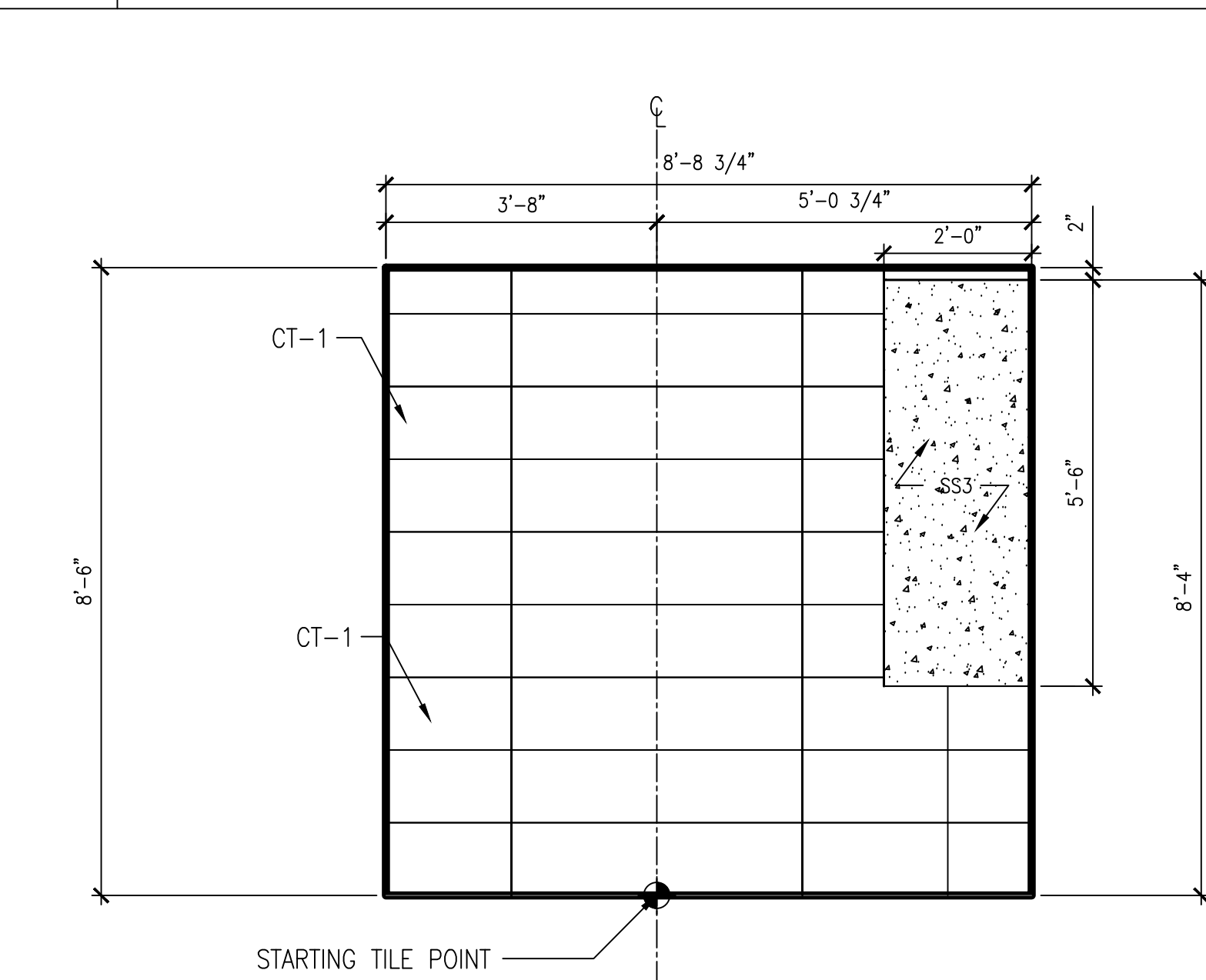
07 1/2"=1'-0" ELEVATIONS: WEST
