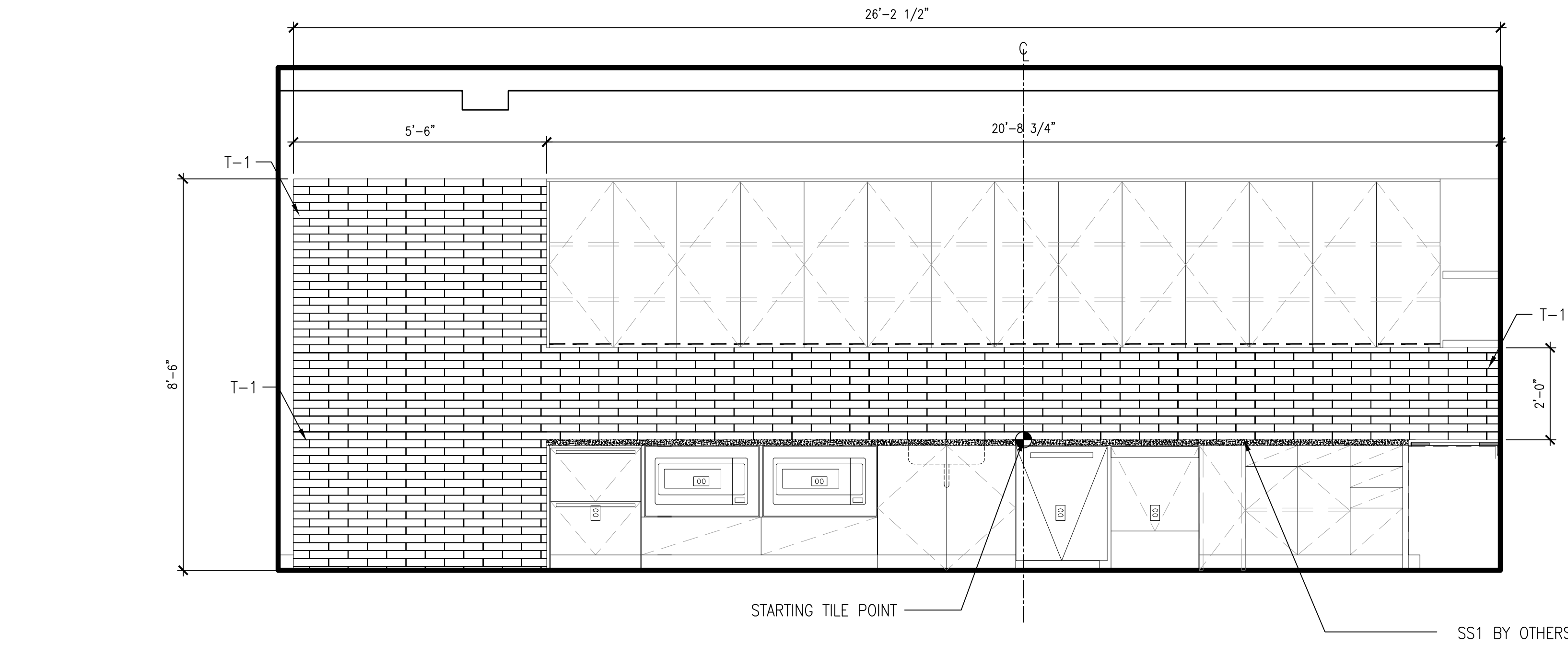
02 1/2"=1'-0" ELEVATION: EAST
