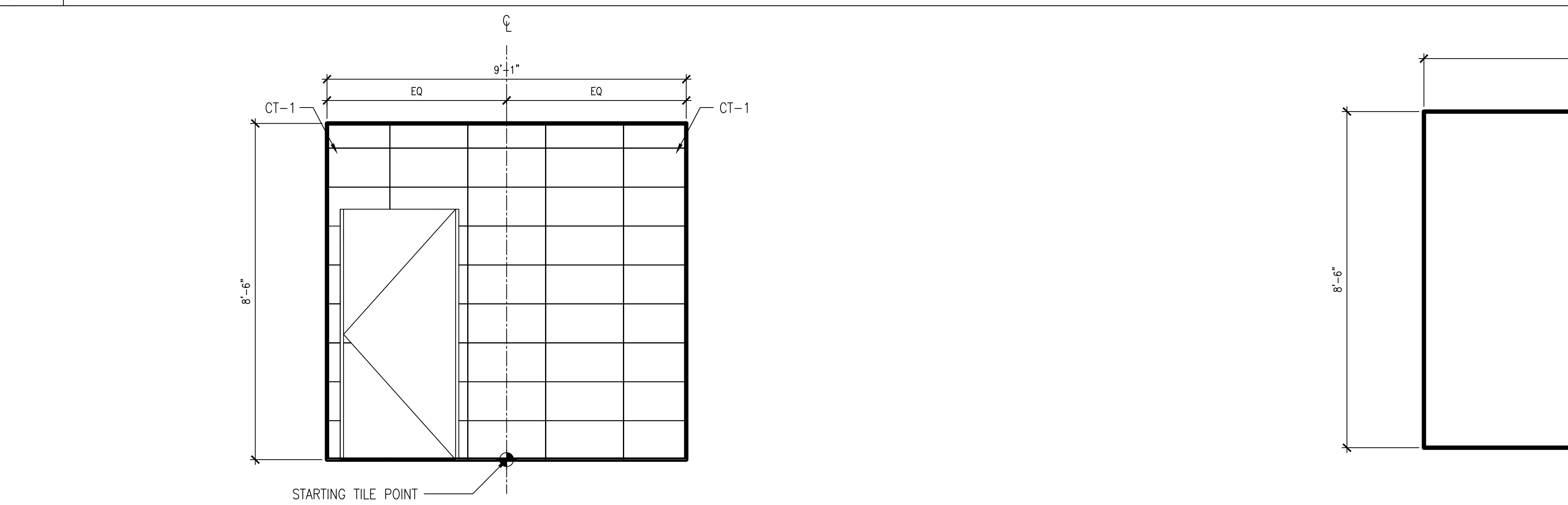
04 1/2"=1'-0" ELEVATION: EAST
