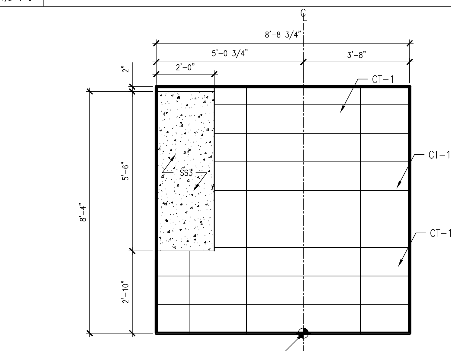
07 1/2"=1'-0" ELEVATION: WEST
