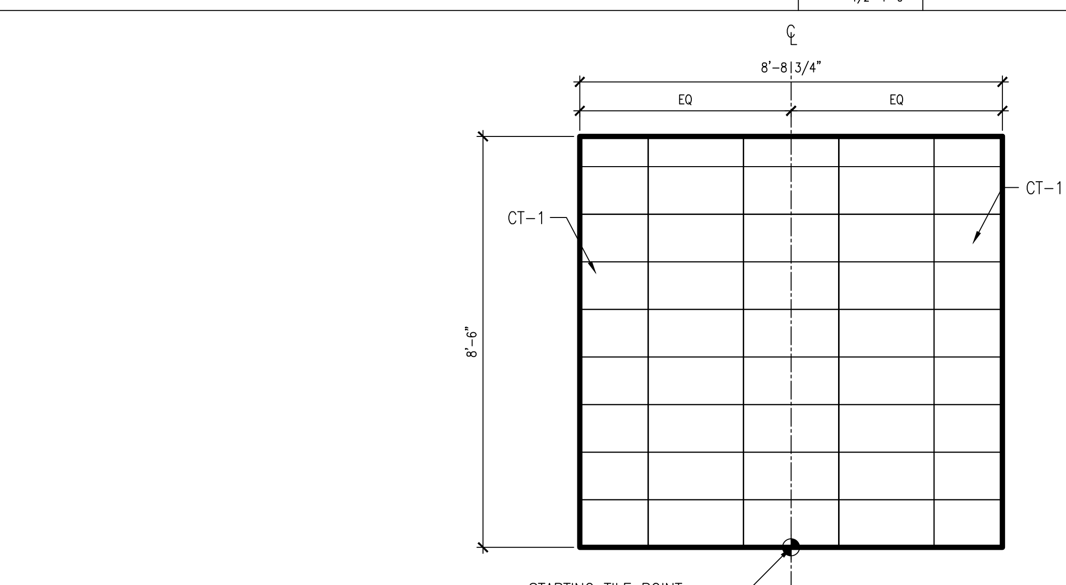
09 1/2"=1'-0" ELEVATION: EAST
